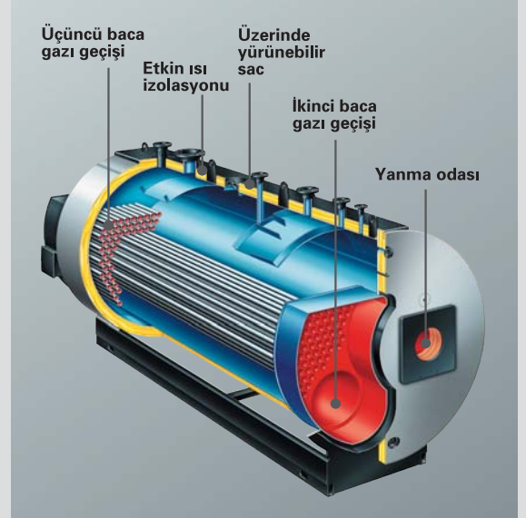
Vitomax 200 WS 1750 - 11630 kW
